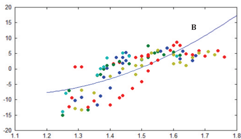
Figure [4]: temperature deviation curve for soil sample B. At suitable phase angle \frac{H}{S} and the annual amplitude of the surface soil temperatures is within the range -120 < A_o > 120
