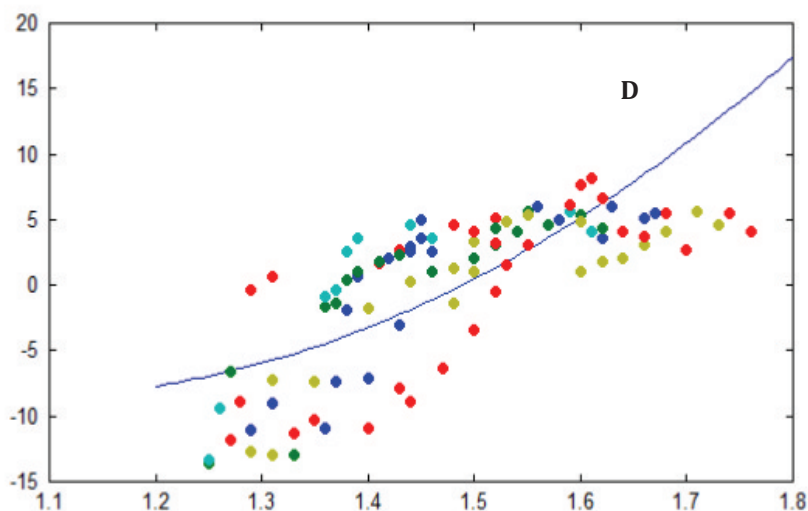
Figure [6]: temperature deviation curve for soil sample D. At suitable phase angle \frac{\pi}{\omega} and the annual amplitude of the surface soil temperatures is within the range -120 < A_o > 120
