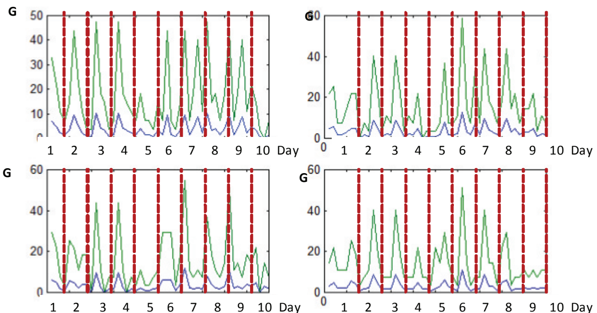
Figure [2]: daily soil heat flux for the four soil samples
